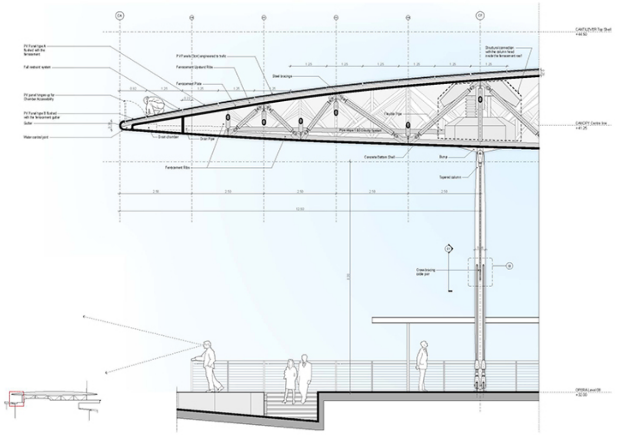
Stavros Niarchos Foundation Cultural Center Athens, Greece Renzo Piano Building Workshop Cantilever Detail Section
